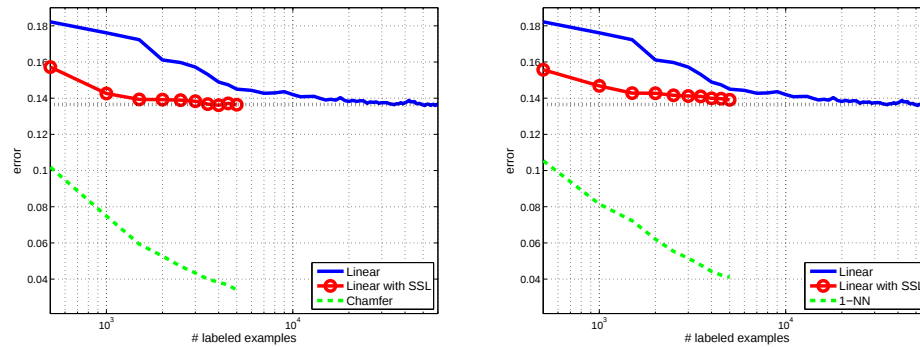
Figure 1. Test error of different algorithms (see description in the text) as a function of the number of labeled examples.
