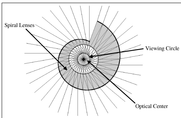
Fig. 19. A spiral shaped lens. The diacaustic of the lens' outer curve is a circle (the viewing circle). Capturing the panorama can be done by an omnidirectional camera at the center of the viewing circle.
