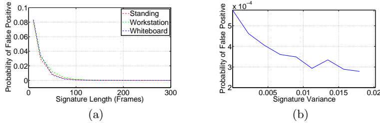
Fig. 7. (a) Average probability of false positive for various signature length corresponding to observer’s signature obtained from different sequences. The false positive probability is non-zero for short signatures but quickly goes to 0 for signatures longer than 100 frames. In our implementation we use signatures of length more than 200. (b) Probability of false positive with respect to signatures of different variance. The length of the signature chosen in this case is 100. The probability is practically zero even for signatures with low variance.
