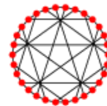
Levi graph
