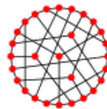
Coxeter graph
