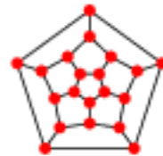
dodecahedral graph
