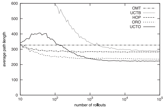
Figure 2: Average travel cost as a function of rollout number for benchmark instance 50-9.
