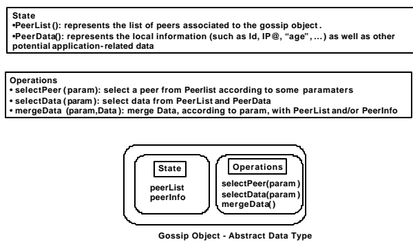
Figure 2: Generalized Implementation of a Gossip Object
