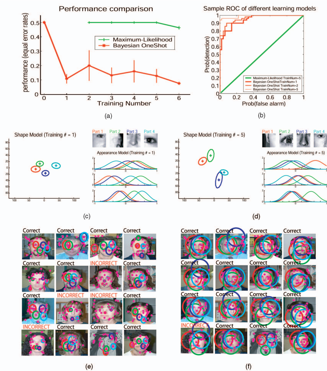
Fig. 7. Summary of face model. (a) Test performances of the algorithm given 0 – 6 number of training image(s) (red line). Zero number of training images is when only the prior model is used. Note the prior alone is not sufficient for categorization. Each data point is obtained by 10 repeated runs with different randomly drawn training and testing images. Error bars show one standard deviation from the mean performance. This result is compared with the maximum-likelihood (ML) method (green). Note that ML cannot learn the degenerate case of a single training image. (b) Sample ROC curves for the Bayesian One-Shot algorithm (red) compared with the ML algorithm (green line). The curves shown here use typical models drawn from the repeated runs summarized in (a). (c), (d), (e), and (f) show typical models learned with one and five training images. (c) Shape model, appearance samples, and appearance densities (of the first three descriptors) for a model trained on one image. (e) Sample foreground test images for the model shown in (c). (d) and (f) correspond to a model trained on five images. Note that the size of the open circles on (e) and (f) indicates the strength of the hypothesis (scaled according to the log likelihood score), not the variance of the part locations. In other words, the bigger the circles, the stronger the algorithm believes in the recognition decision. Only the mean locations of the parts are shown here in pink dots. (c) Model from one training example. (d) Model from five training example. (e) Testing examples from model in (c). (f) Testing examples from model in (d).
