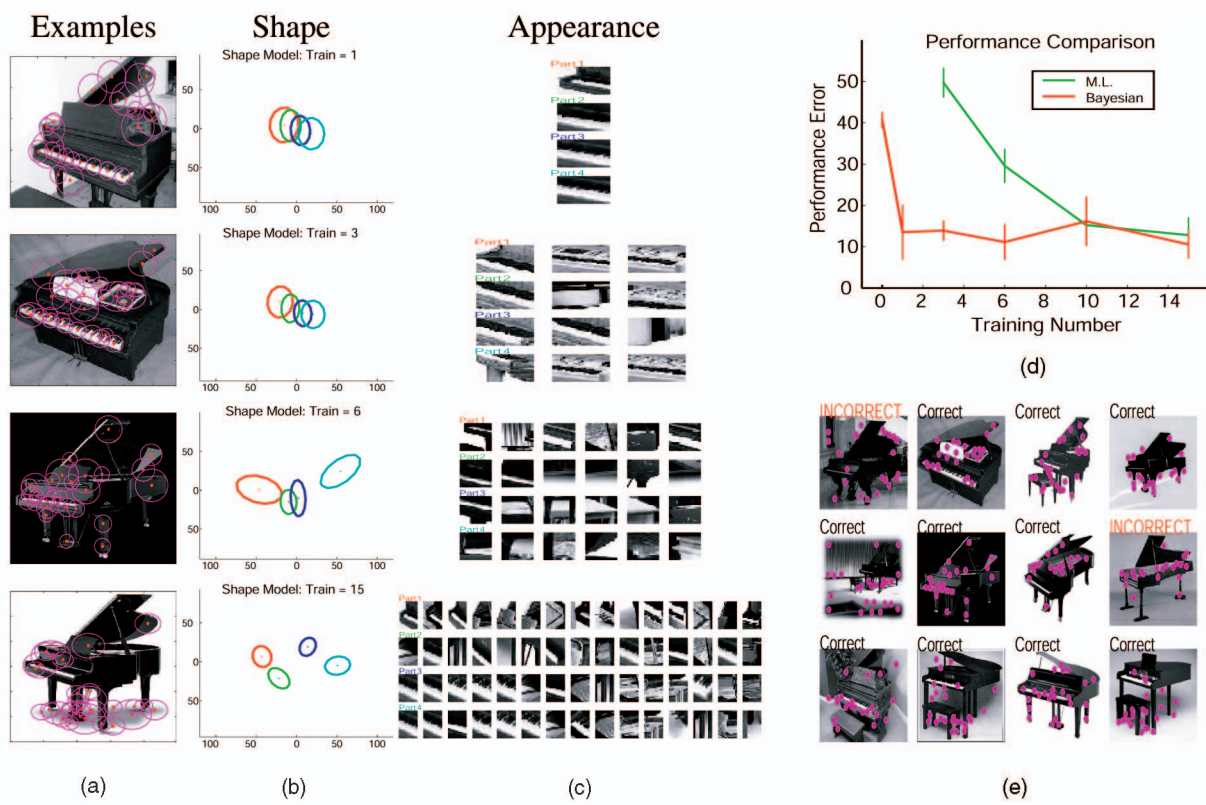
Fig. 10. Results for the “grand-piano” category. Column 1 shows examples of feature detection. Column 2 shows the shape models learned from \{1, 3, 6, 15\} training images. Column 3 shows the appearance patches for the model learned from \{1, 3, 6, 15\} training images. The top panel of Column 4 shows the comparative results between ML and Bayesian methods (the error bars show the variation over the 10 runs). The bottom panel of Column 4 shows the recognition result for the Bayesian One-Shot algorithm for one training image. Pink dots indicate the center of detected interest points.
