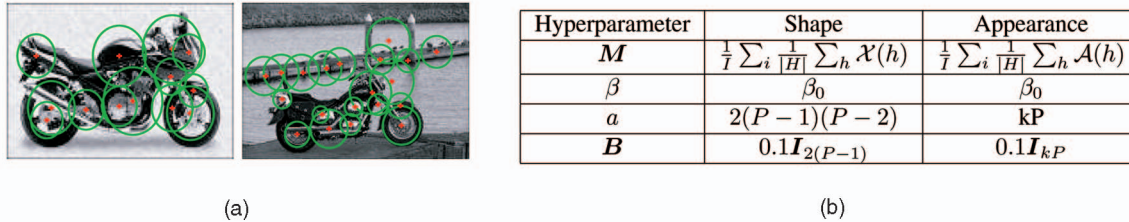
Fig. 3. (a) Sample training images for the motorbike category, with the output of the feature detector overlaid. (b) Initial values of the hyperparameters of the parameter posterior for shape and appearance.
