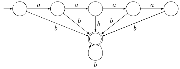
Figure 3 A DFA for L_4 .
