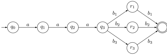
Figure 2 A DFA for L_3 .
