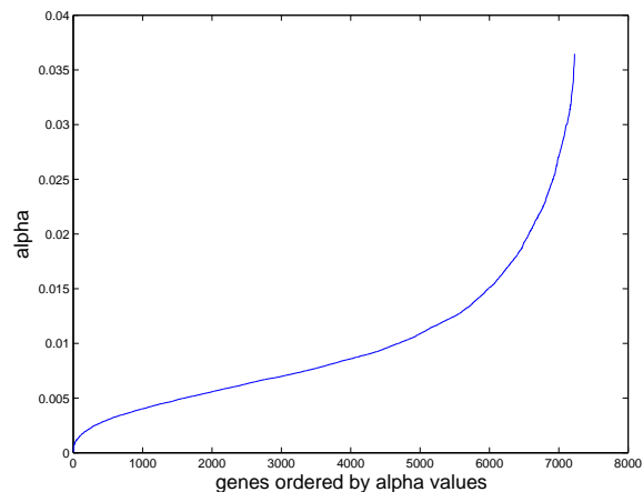
Figure 2: A plot of the sorted \alpha -values for the Hematopoietic differentiation cell lines. As noted, all values come out positive despite the fact that positivity is not explicitly constrained in the energy function. The profile of the values indicates sparsity meaning that around 95% of the values are of an order of magnitude smaller than the remaining 5%.
