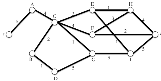
Figure 1: A WLG with a nonempty core
