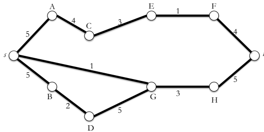
Figure 2: A WLG with an empty core
