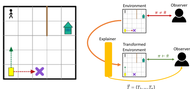
Figure 1: Reinforcement Learning Policy Explanation model (Right), and Taxi domain example (Left) where the agent’s anticipated policy depicted by the green arrow, and the actual one by the red arrow.
