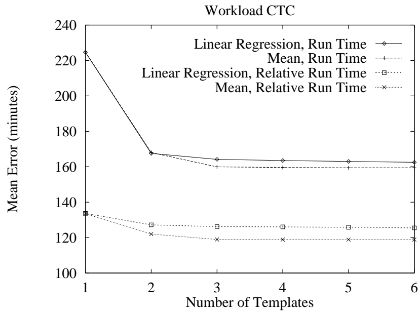
Fig. 1. Mean errors of ANL and CTC greedy searches
