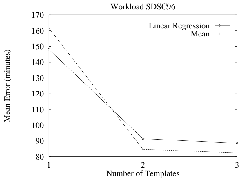
Fig. 2. Mean errors of SDSC greedy searches
