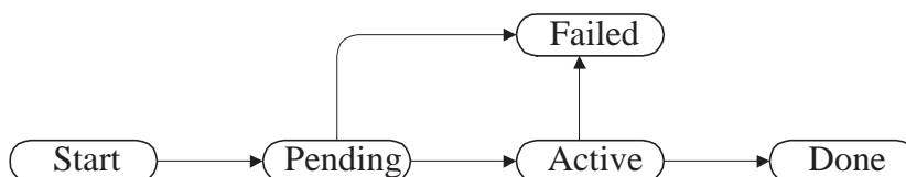
Fig. 5. State transition diagram for resource allocation requests submitted to the GRAM resource management API
