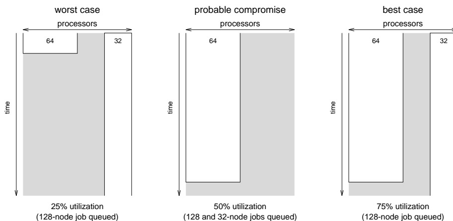
Fig. 1. Example of the problems faced by variable partitioning.
