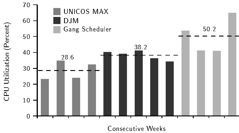
Fig. 10. Weekly utilization with the three schedulers. Dashed lines and numbers denote averages.
