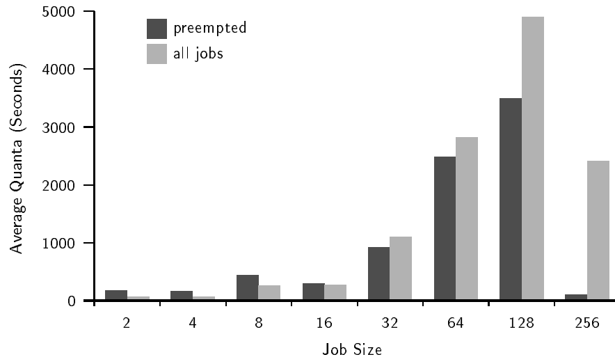
Fig. 15. Average time quanta for different size jobs.
