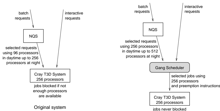
Fig. 7. The place of the gang scheduler in the Cray T3D scheduling system.
