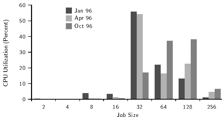
Fig. 9. Changes in workload distribution due to use of the Gang Scheduler.
