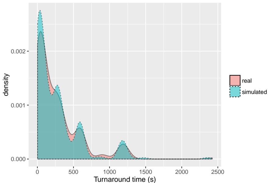
Fig. 9. The density of the turnaround time for jobs of workload ( seed = 1, psize = 37 ).
