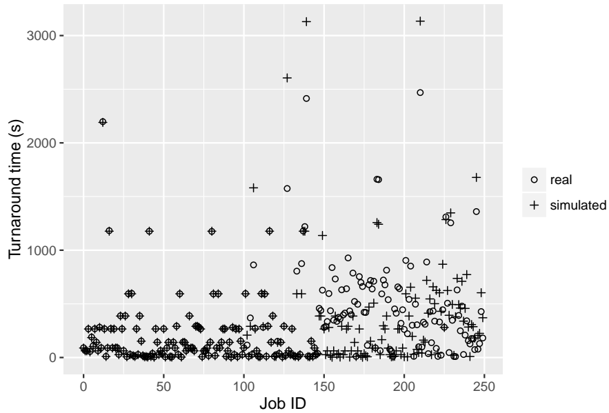
Fig. 7. The turnaround time for jobs of workload ( seed = 4, psize = 37 ).
