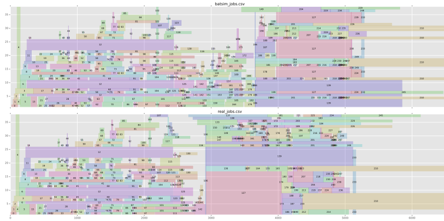
Fig. 4. The time-resource Gantt chart of workload ( seed = 4, psize = 37 ).
