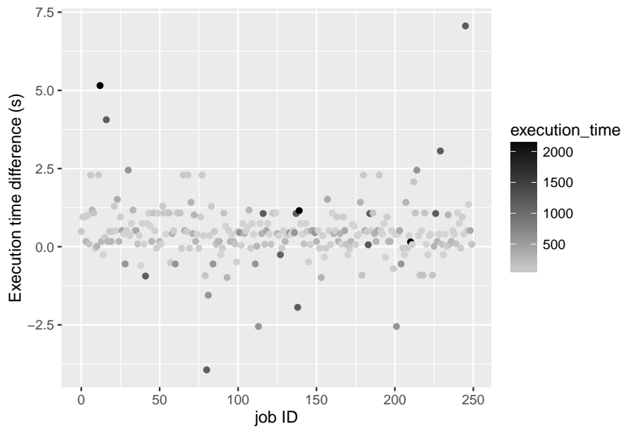
Fig. 5. The difference between the real and the simulated execution time for all the jobs in workload ( seed = 4, psize = 37 ).
