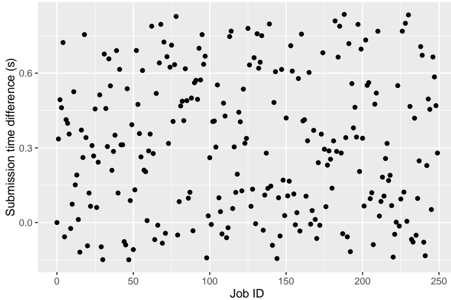
Fig. 6. The difference between the real and the simulated submission time of the jobs in workload ( seed = 4, psize = 37 ).
