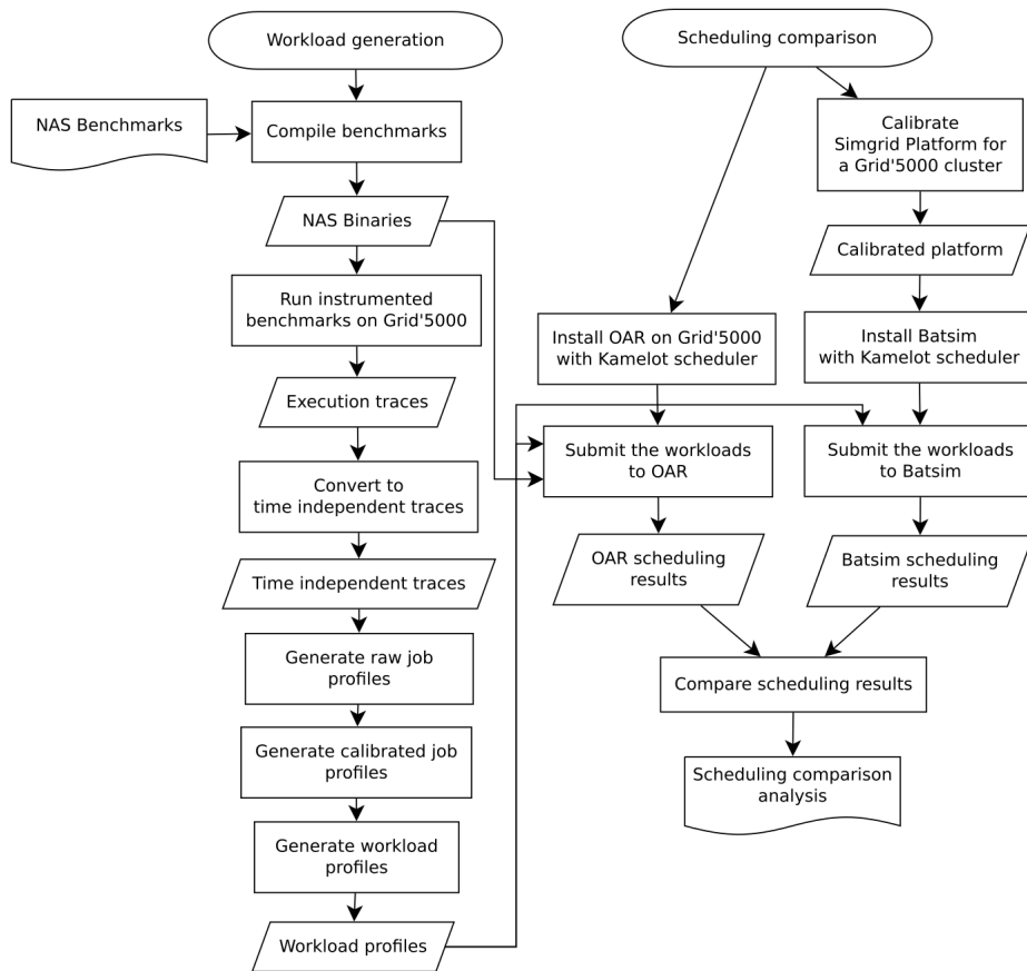
Fig. 3. Simplified workload generation experiment workflow.
