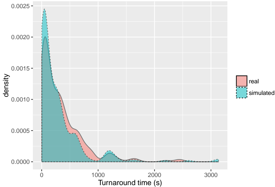
Fig. 8. The density of the turnaround time for jobs of workload ( seed = 4, psize = 37 ).
