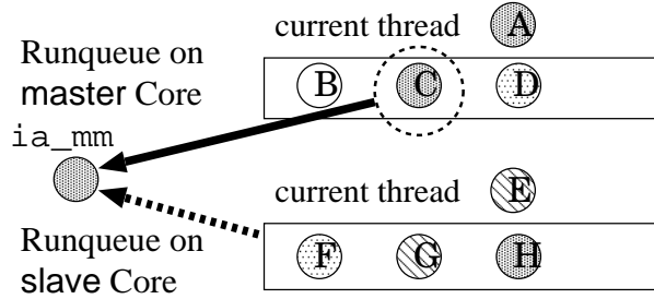
Fig. 3. Example case of IAS. When sibling threads (circles with the same pattern) are aggregated in Core 0 by TAS, the memory address space of the sibling thread is registered in ia_mm . The scheduler on Core 1 looks for threads sharing the same memory address space with ia_mm and considers the thread as the candidate for the next thread.
