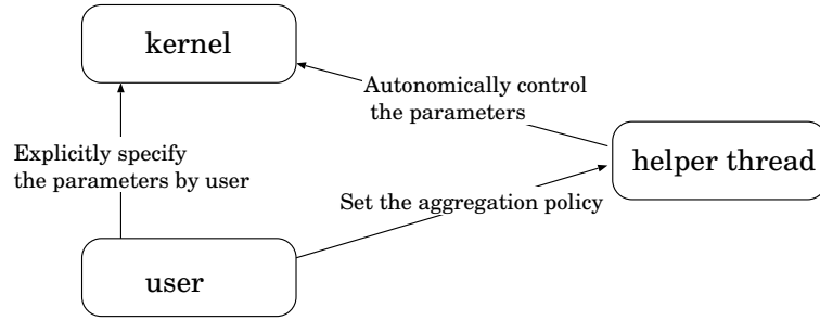
Fig. 1. The overview of the scheduling mechanism. We divide the scheduling functions into three domains, which enables the dynamic and flexible control of thread aggregation. In this paper, we focus on User domain.
