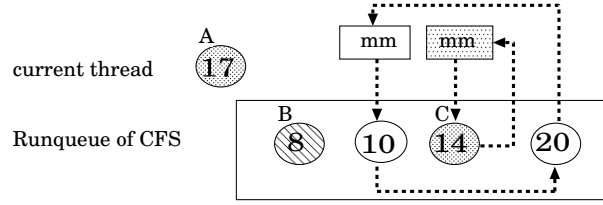
Fig. 2. Example case of TAS. A circle represents a thread and the pattern inside the circle expresses its memory address space. TAS looks for the sibling thread of the current thread from the list of the sibling threads. If there exists a sibling thread (thread C), TAS considers the thread as the candidate for the next thread.
