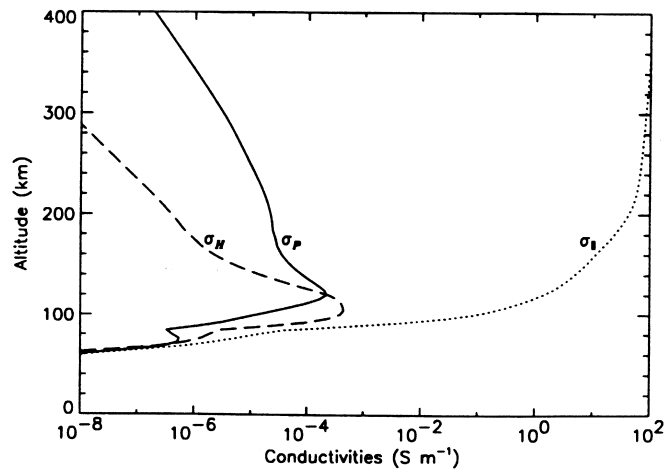
Figure 6: Typical noontime parallel ( \sigma_0 ), Pedersen ( \sigma_1 ) and Hall ( \sigma_2 ) conductivities at 44.6^\circ\text{N} , 2.2^\circ\text{E} for solar minimum conditions on March 21. The different types of conductivity characterize the behavior of the ionosphere as a reflector of ELF waves. Adapted from A. D. Richmond, in H. Volland (editor), 'Handbook of Atmospheric Electrodynamics', CRC Press 1995, with permission. (CRC Press Home Page http://www.crcpress.com ).
