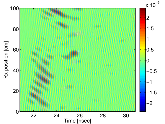
Fig. 6. An example of measured impulse responses in the 5-6 GHz band. This example is non line of sight, with terminal separation of about 6.8 meters, the terminals were located at different floors of the same building. The figure shows pass-band impulse responses measured over a one-meter rail with receiver positions separated by 2 mm. The vertical axis represents positions along the rail, the receiver was located closer to the transmitter at the top part of the picture than at its bottom. The carrier frequency (5.5 GHz in this case) was not removed in order to not lose the angle of arrival information, so the impulse response is real and shows a strong 5.5 GHz oscillation.
