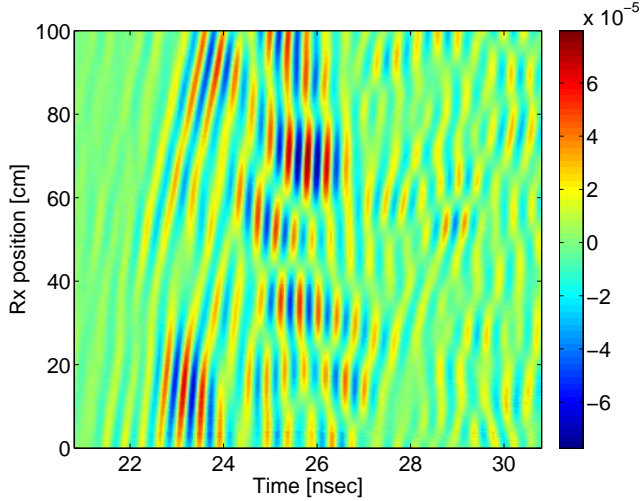
Fig. 7. An example of measured impulse responses in the 2-3 GHz band, a higher bands of the same measurement is shown in Figure 6. Note that the diagonal features (that correspond to multipath components) are longer in this band than in the higher band. See comments below Figure 6.
