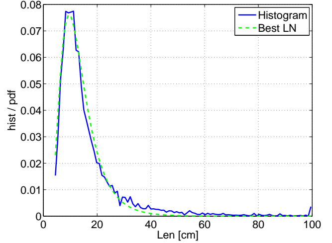
Fig. 5. A histogram of the length of extracted MPCs that account for 80% of the channel response energy, shown with the best fit log-normal distribution that has mean 13.6 cm and standard deviation 7.1 cm. The visibility length statistics (mean and standard deviation) over all extracted MPCs is are different from the statistics averaged over individual measurements.
