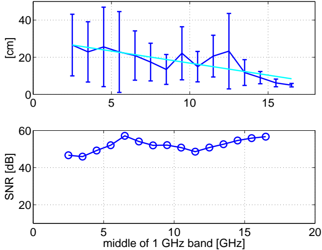
Fig. 8. The average spatial length of multipath components accounting for 80% of the measured response energy from a single typical measurement and the standard deviation, plotted in the top graph against sub-band carrier frequency. The signal to noise ratio (SNR) is indicated in the bottom graph.
