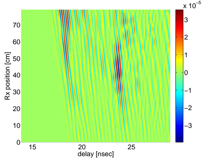
Fig. 1. An example of measured impulse responses. The horizontal axis has delay and the vertical receiver positions. The responses are real with amplitudes that are shown in color. This measurement was taken with terminal separation of 9.8 m, and is typical of near line of sight situations. The color reflects linear amplitude values that may be negative.
