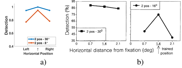
Figure 4. Results of testing the trained network with the same discrimination task, but where the odd element was shifted to a different location from the trained one. a) CNN network. b) A qualitatively similar phenomenon was reported in [2] Fig. 2c.
