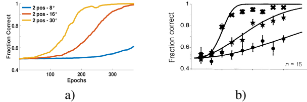
Figure 2. Results of training to perform the relevant discrimination task with a few levels of difficulty. a) CNN network: the difficulty level is controlled by the angle difference between the odd line segment and the background segments: 8^\circ , 16^\circ , 30^\circ . b) [2] Fig. 1b. The two plots show qualitatively similar behavior - longer training time for more difficult discrimination tasks. We note, however, that both difficulty level and improvement were measured quite differently in a) and b).
