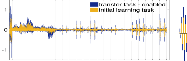
Figure 12. Left. Visualization of the weights of the trained network: blue bars show the weights at the end of the process, and super-imposed yellow bars show the intermediate weights after training with the initial easy (high SNR) task. Almost all weight changes correspond to amplification (more positive or more negative values); very few changes correspond to decrease of absolute value or change of sign. Right. To demonstrate this point, we show a close-up on a part of the plot, focusing on the changes in a few of the final weights going from channels to decision neurons. This is typical of all the other weight changes in the network.
