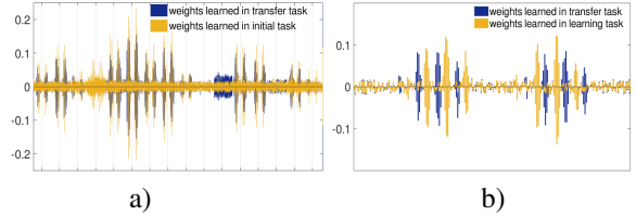
Figure 9. a) The weights of the connections between the last conv-pool layer and the output neurons. Faint vertical line separate the weights into 16 groups, each corresponding to weights originating from one channel in the last conv-pool layer. The intermediate weights (yellow) are super-imposed on the final weights (blue). Since the intermediate weights hardly changed in the second phase of training, the final weights are in fact described by the union of the yellow and blue bars. b) Close-up on a typical channel, showing only weights originating from one of the channels in the last conv-pool layer.
