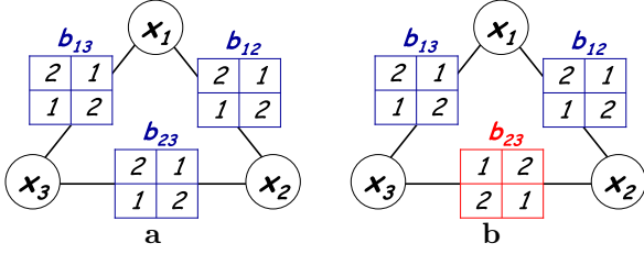
Figure 3: An illustration of a frustrated cycle. The tables show pairwise beliefs obtained by a convex BP algorithm. For the three nodes in (a), it is possible to find an assignment x^* that maximizes the pairwise and singleton beliefs. Theorem 1 proves that this means that x^* is the global optimum. For the three nodes in (b) it is impossible to find such an assignment.
