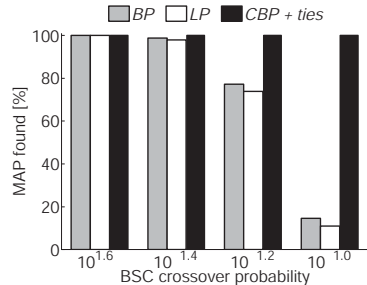
Figure 5: A comparison of success rates as a function of crossover probability for a LDPC code on a binary symmetric channel. Each bar represents 400 trials.
