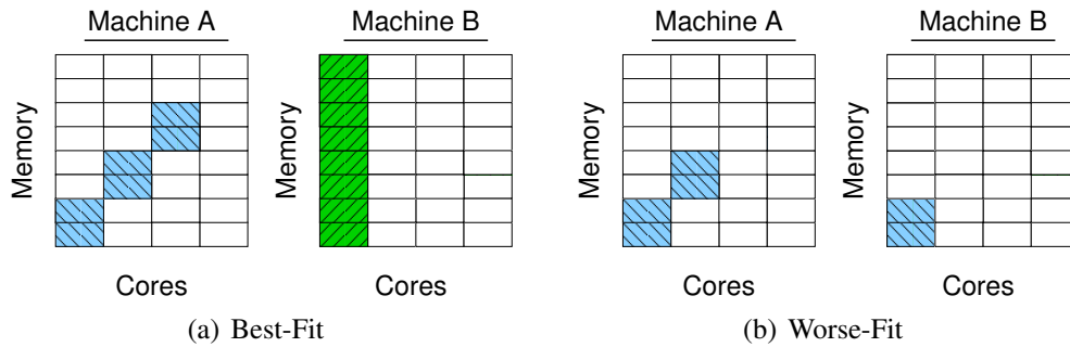
Figure 3.2: Scenario for which Best-Fit (left) is better than Worse-Fit (right).
