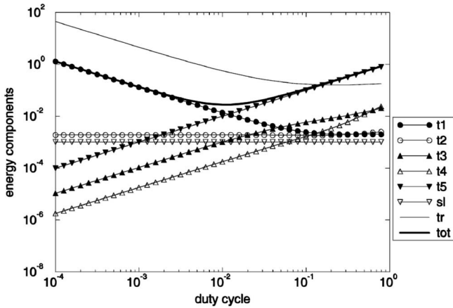
Fig. 6. Components of the normalized average energy consumption versus duty cycle. N = 50 , network load 0.1.
