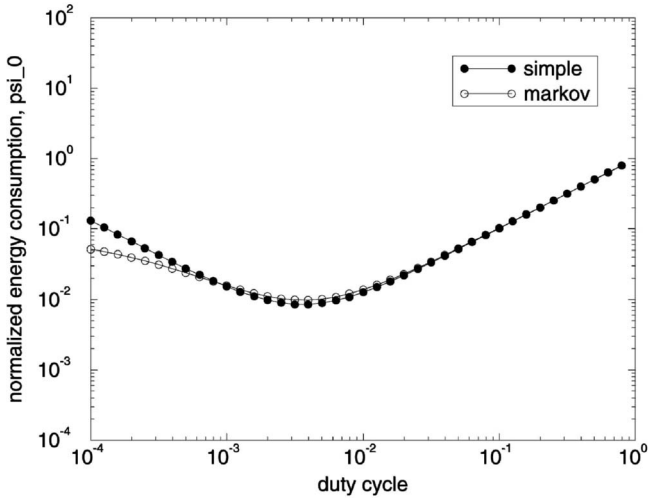
Fig. 14. Normalized average energy consumption, \psi_0 , versus duty cycle. Simple analysis and semi-Markov model compared. N = 50 , network load 0.01.
