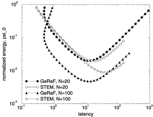
Fig. 3. Average normalized energy consumption, \psi_0 , versus latency (in units of T_D ). GeRaF and STEM compared. N = 20, 100 , network load 0.01.
