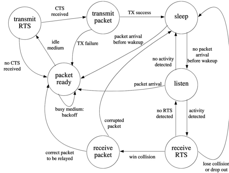
Fig. 12. Transition diagram of the semi-Markov model for GeRaF.
