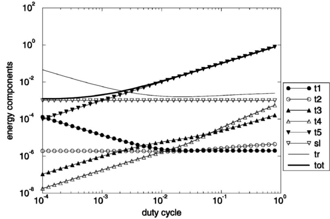
Fig. 7. Components of the normalized average energy consumption versus duty cycle. N = 500 , network load 0.001.
