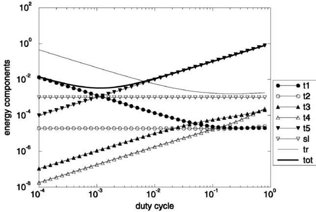
Fig. 5. Components of the normalized average energy consumption versus duty cycle. N = 50 , network load 0.001.
