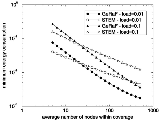
Fig. 8. Optimal normalized average energy consumption, \psi , versus average number of nodes within coverage, N . Network load 0.01 and 0.1.
