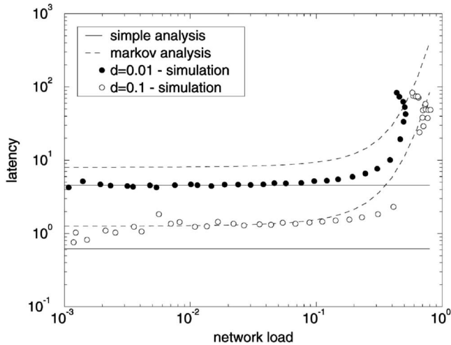
Fig. 17. Latency (in units of T_D ) versus the network load. Simple analysis and semi-Markov model compared with simulation points. N = 50 , duty cycle 0.01 and 0.1.
