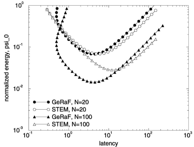
Fig. 4. Average normalized energy consumption, \psi_0 , versus latency (in units of T_D ). GeRaF and STEM compared. N = 20, 100 , network load 0.1.
