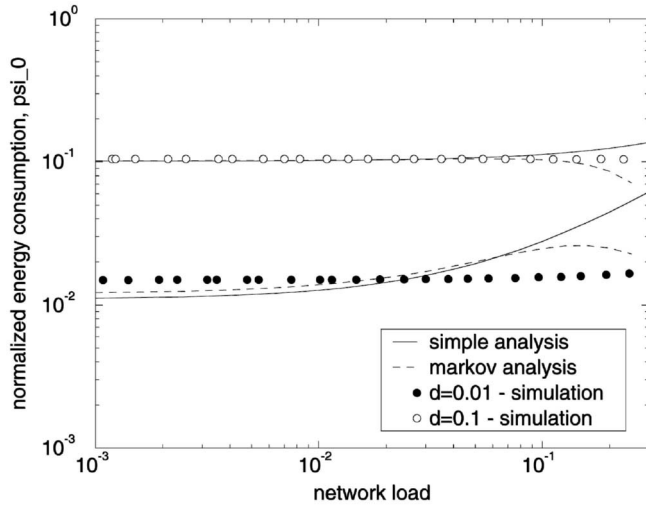
Fig. 16. Normalized average energy consumption, \psi_0 , versus the network load. Simple analysis and semi-Markov model compared with simulation points. N = 50 , duty cycle 0.01 and 0.1.
