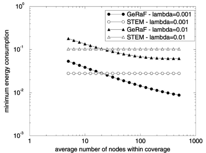
Fig. 10. Optimal normalized average energy consumption, \psi , versus average number of nodes within coverage, N . Traffic per node \lambda = 0.001 and 0.01.
