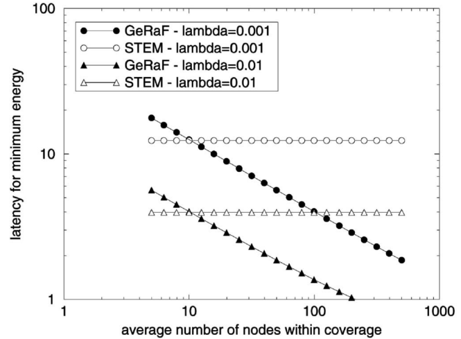
Fig. 11. Latency (in units of T_D ) corresponding to optimal energy consumption versus average number of nodes within coverage, N . Traffic per node \lambda = 0.001 and 0.01.
