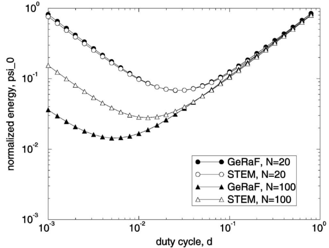
Fig. 2. Average normalized energy consumption, \psi_0 , versus duty cycle, d . GeRaF and STEM compared. N = 20, 100 , network load 0.1.
