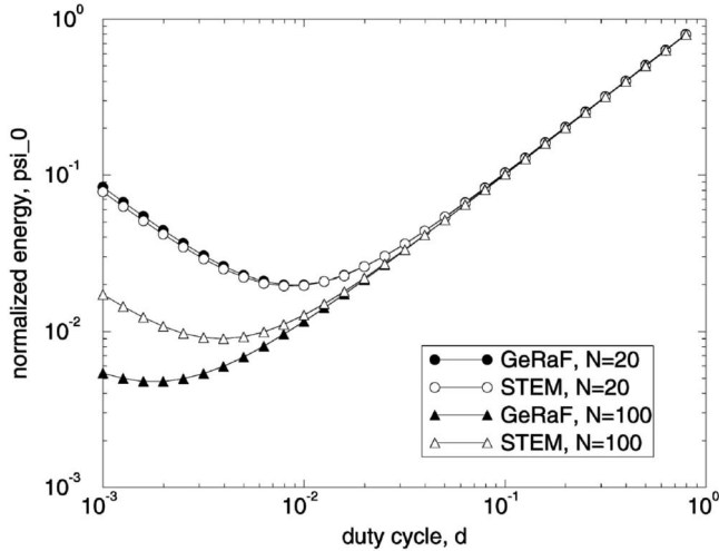
Fig. 1. Average normalized energy consumption, \psi_0 , versus duty cycle, d . GeRaF and STEM compared. N = 20, 100 , network load 0.01.
