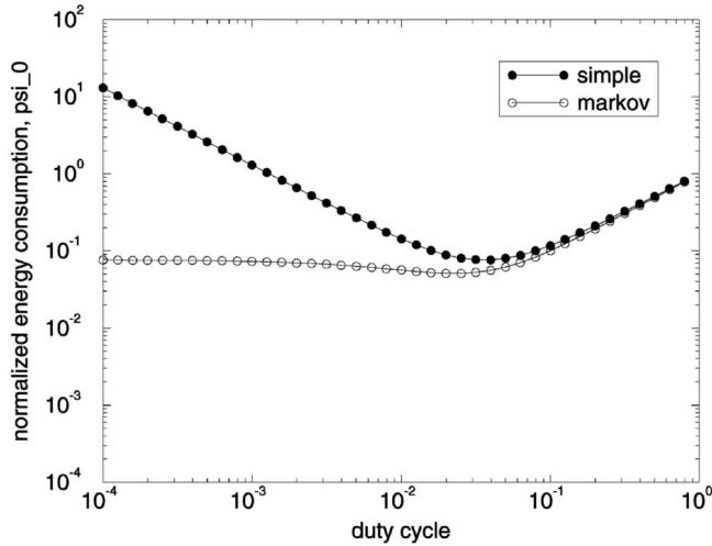
Fig. 13. Normalized average energy consumption, \psi_0 , versus duty cycle. Simple analysis and semi-Markov model compared. N = 5 , network load 0.01.
