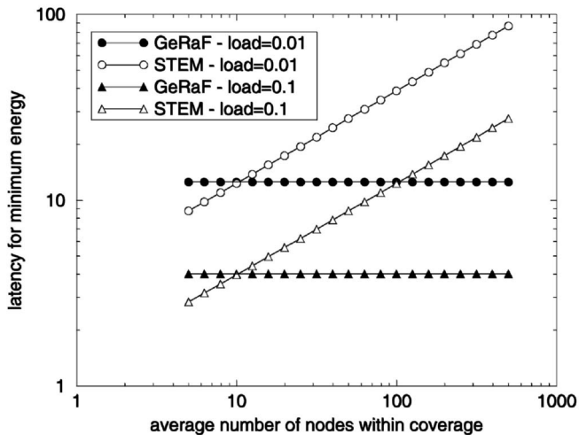
Fig. 9. Latency (in units of T_D ) corresponding to optimal energy consumption versus average number of nodes within coverage, N . Network load 0.01 and 0.1.
