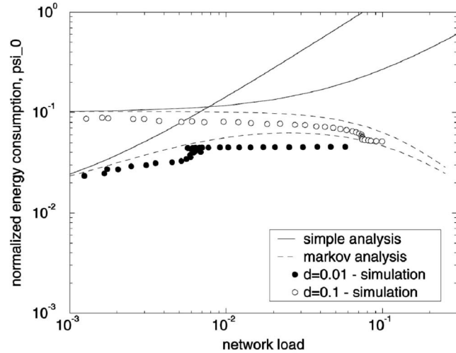
Fig. 15. Normalized average energy consumption, \psi_0 , versus the network load. Simple analysis and semi-Markov model compared with simulation points. N = 5 , duty cycle 0.01 and 0.1.
